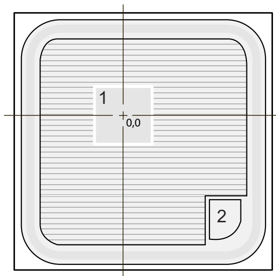
Backside: Drain
