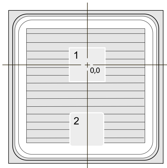
Backside: Drain
