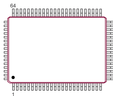
64-Lead PQFP (PG) (top view)
